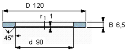
Universal washer
